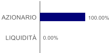
Benchmark
